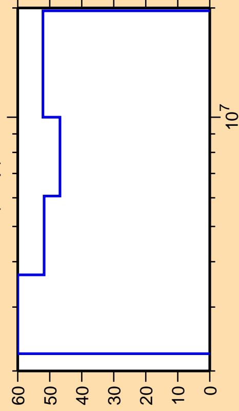
\Delta\sigma/\sigma vs. E for ^{90}\text{Tc}(n,np)
