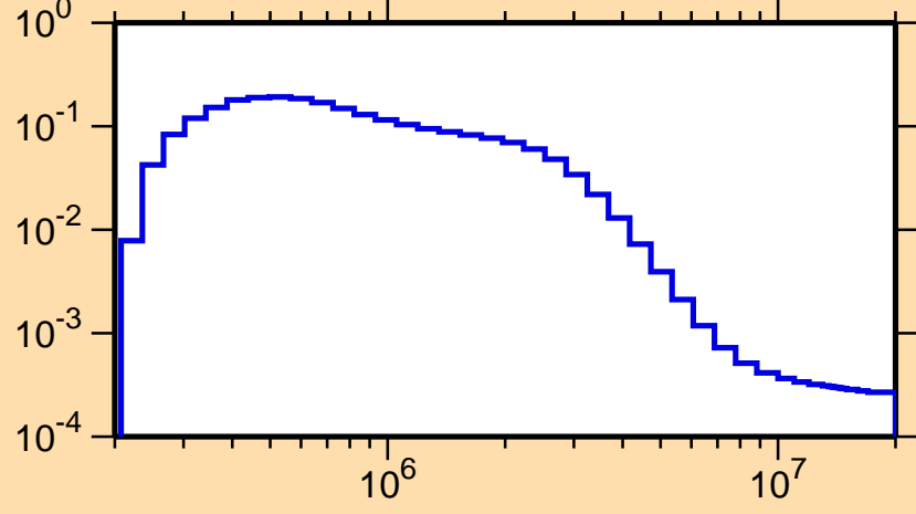
\sigma vs. E for ^{92}\text{Tc}(n,n_1)
