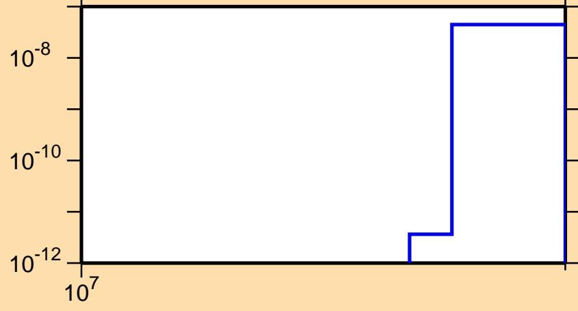
\sigma vs. E for ^{92}\text{Tc}(n,\text{pt})
