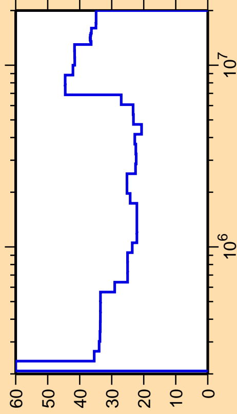
\Delta\sigma/\sigma vs. E for ^{92}\text{Tc}(n,n_1)
