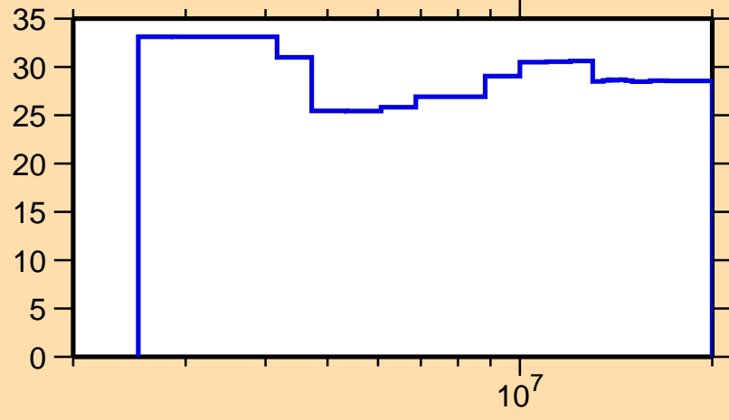
\Delta\sigma/\sigma vs. E for ^{92}\text{Tc}(n,n\text{cont.})
