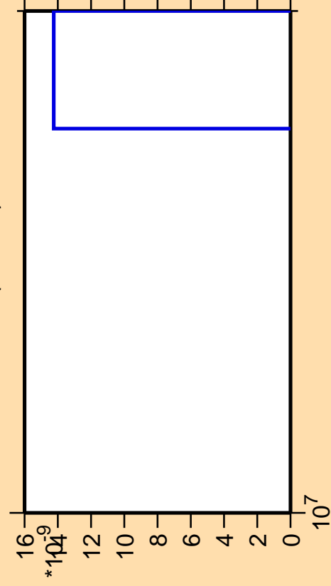
\Delta\sigma/\sigma vs. E for ^{93}\text{Tc}(n,2n\alpha)
