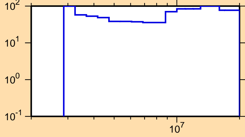
\Delta\sigma/\sigma vs. E for ^{93}\text{Tc}(n,n\text{cont.})
