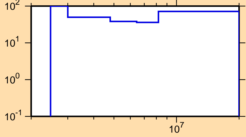
\Delta\sigma/\sigma vs. E for ^{93}\text{Tc}(n,ncont.)
