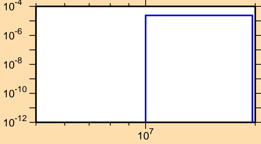
\sigma vs. E for ^{93}\text{Tc}(n,t)
