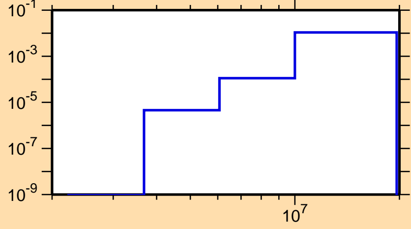
\sigma vs. E for ^{93}\text{Tc}(n,d)
