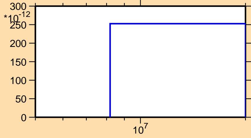
\sigma vs. E for ^{93}\text{Tc}(\text{mt } 45)
