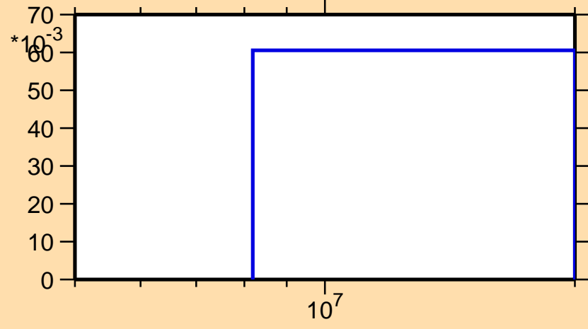
\sigma vs. E for ^{93}\text{Tc}(n,2n)
