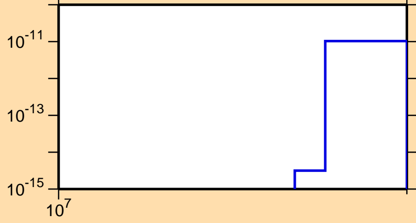
\sigma vs. E for ^{94}\text{Tc}(n,2n\alpha)
