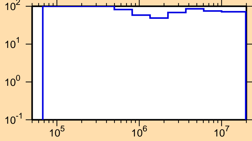
\Delta\sigma/\sigma vs. E for ^{94}\text{Tc}(n,n_1)
