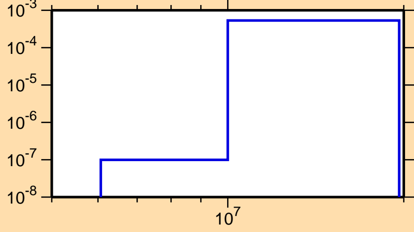
\sigma vs. E for ^{94}\text{Tc}(n,t)
