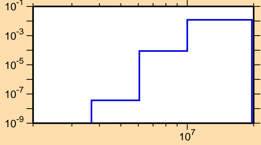
\sigma vs. E for ^{94}\text{Tc}(n,d)
