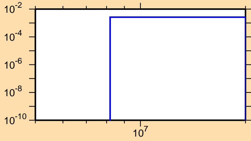
\sigma vs. E for ^{94}\text{Tc}(n,n\alpha)
