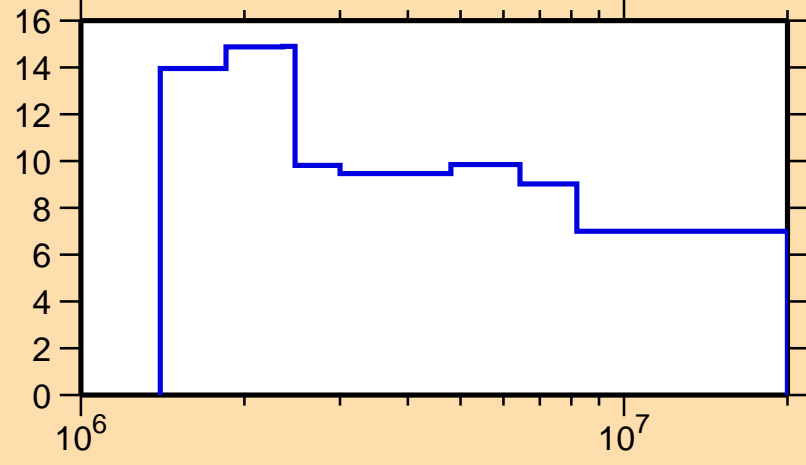
\Delta\sigma/\sigma vs. E for ^{94}\text{Tc}(n, n\text{onel.})
