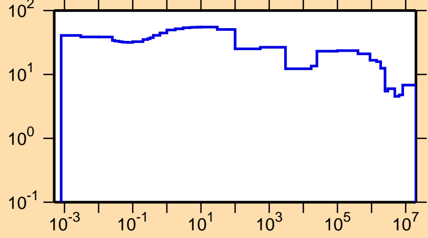
\Delta\sigma/\sigma vs. E for ^{94}\text{Tc}(n,\text{tot.})
