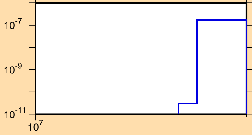
\sigma vs. E for ^{95}\text{Tc}(n,nt)
