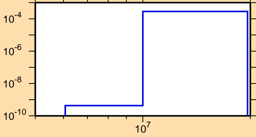
\sigma vs. E for ^{95}\text{Tc}(n,t)
