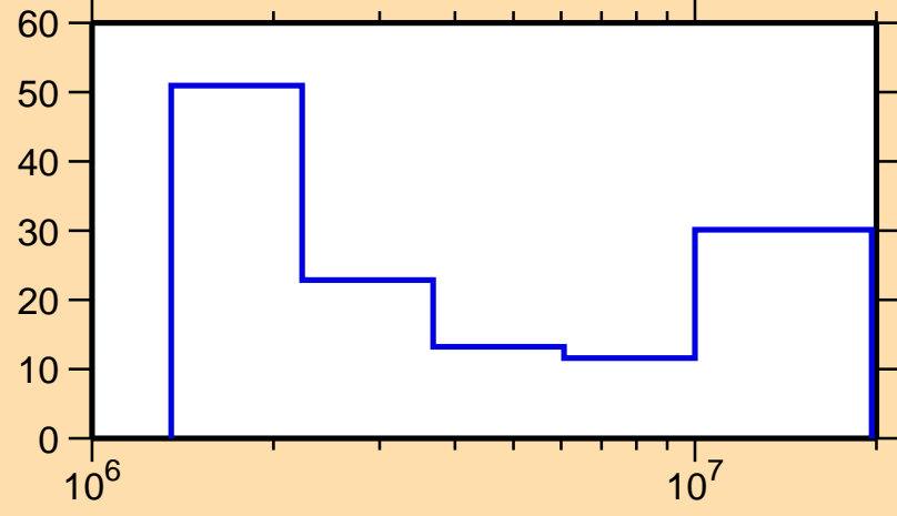
\Delta\sigma/\sigma vs. E for ^{95}\text{Tc}(n,ncont.)
