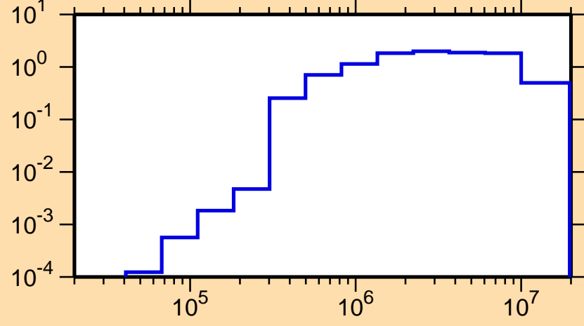
\sigma vs. E for ^{95}\text{Tc}(n,\text{inel.})
