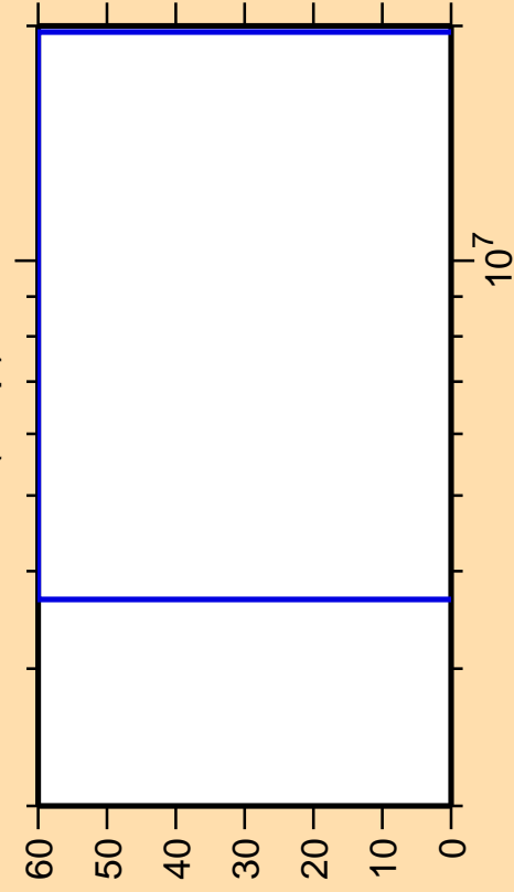
\Delta\sigma/\sigma vs. E for ^{95}\text{Tc}(n,np)
