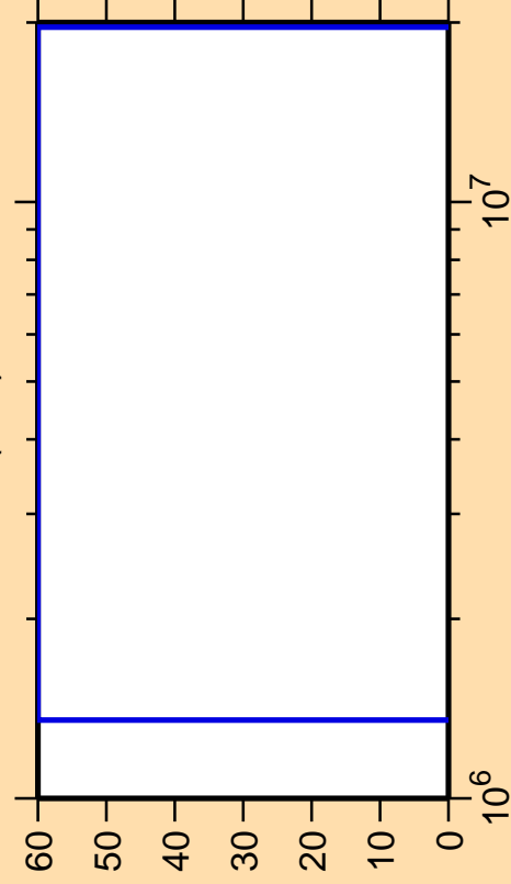
\Delta\sigma/\sigma vs. E for ^{95}\text{Tc}(n,\alpha)
