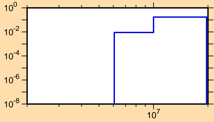
\sigma vs. E for ^{95}\text{Tc}(n,np)
