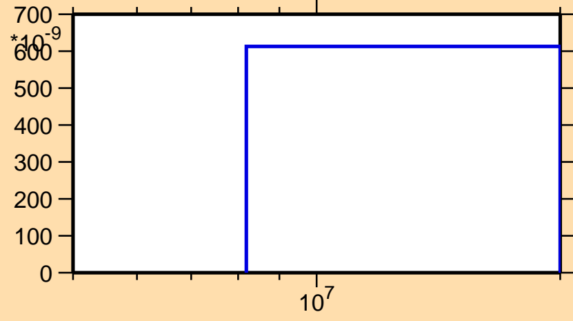
\sigma vs. E for ^{95}\text{Tc}(n,nd)
