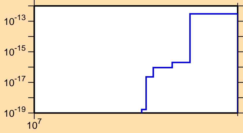
\sigma vs. E for ^{95}\text{Tc}(\text{mt } 34)
