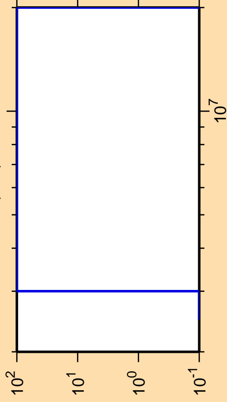
\Delta\sigma/\sigma vs. E for ^{95}\text{Tc}(n,d)
