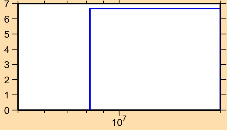
\Delta\sigma/\sigma vs. E for ^{95}\text{Tc}(n,\text{nonel.})
