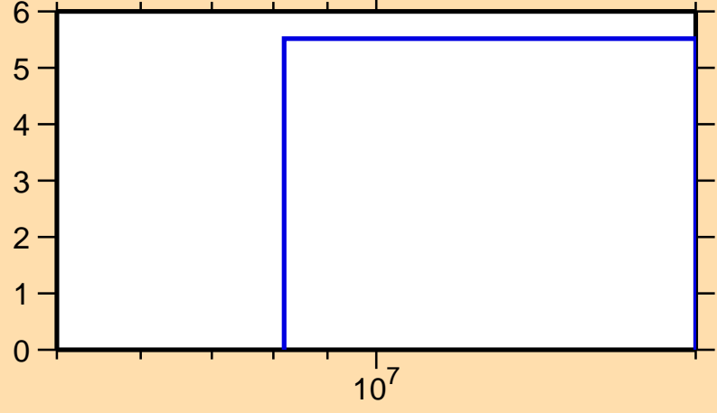
\Delta\sigma/\sigma vs. E for ^{95}\text{Tc}(n,\text{tot.})
