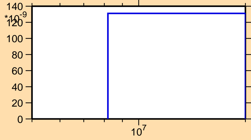
\sigma vs. E for ^{95}\text{Tc}(n,\text{He3})
