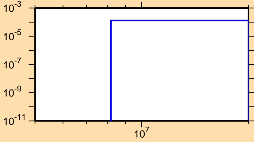
\sigma vs. E for ^{95}\text{Tc}(n,t)
