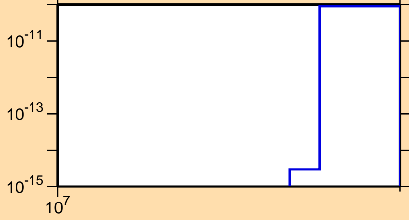
\sigma vs. E for ^{96}\text{Tc}(n,\text{pt})
