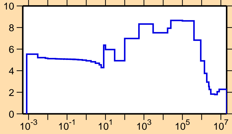
\sigma vs. E for ^{96}\text{Tc}(n,\text{el.})
