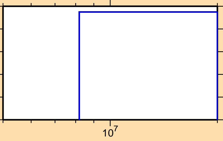
\sigma vs. E for ^{96}\text{Tc}(n,nt)
