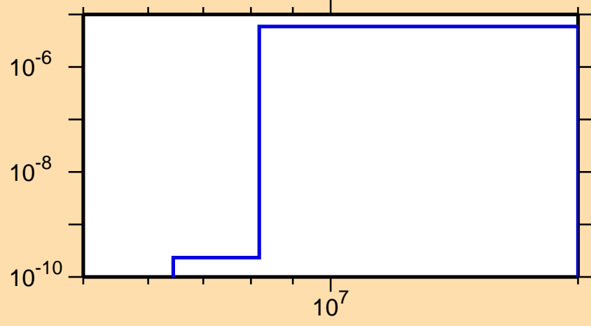
\sigma vs. E for ^{96}\text{Tc}(n,p\alpha)
