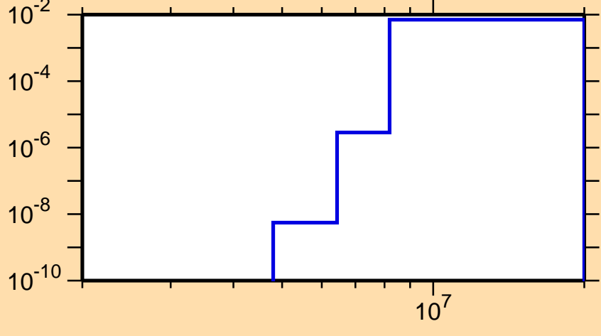
\sigma vs. E for ^{96}\text{Tc}(n,d)
