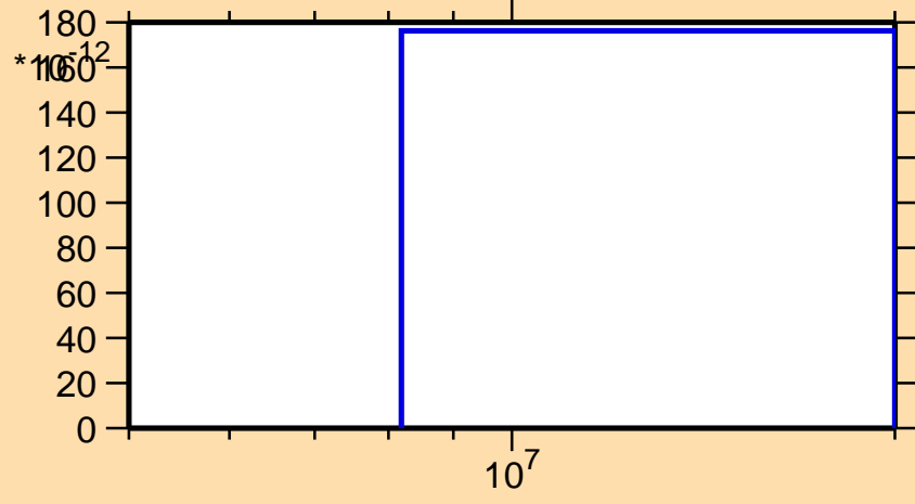
\sigma vs. E for ^{96}\text{Tc}(\text{mt } 45)
