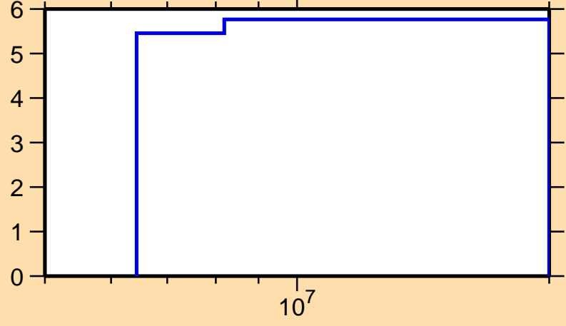
\Delta\sigma/\sigma vs. E for ^{96}\text{Tc}(n,\text{nonel.})
