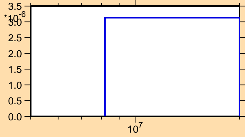
\sigma vs. E for ^{96}\text{Tc}(n,nd)
