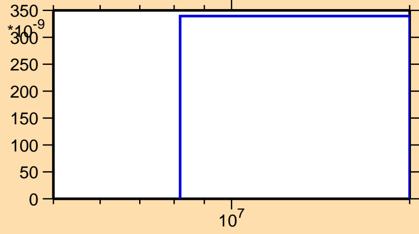
\sigma vs. E for ^{96}\text{Tc}(n,\text{He3})
