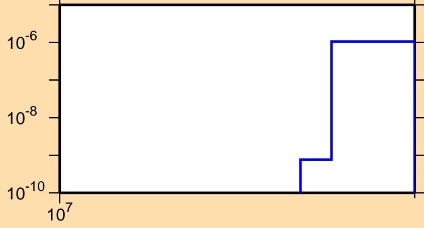
\sigma vs. E for ^{96}\text{Tc}(n,nt)
