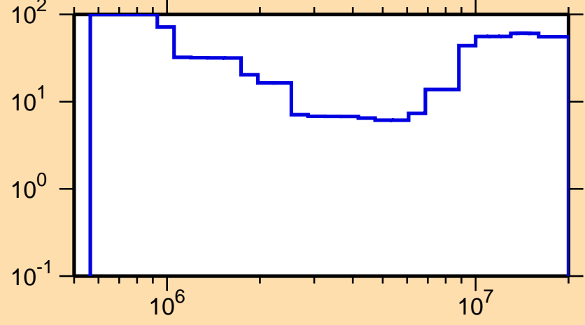
\Delta\sigma/\sigma vs. E for ^{96}\text{Tc}(n,ncont.)
