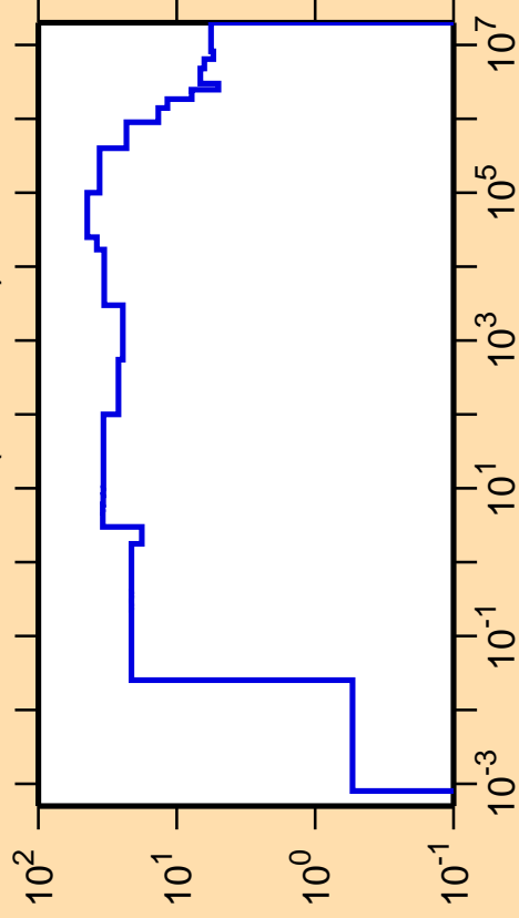
\Delta\sigma/\sigma vs. E for ^{96}\text{Tc}(n,\text{nonel.})
