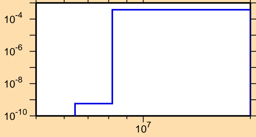
\sigma vs. E for ^{96}\text{Tc}(n,t)
