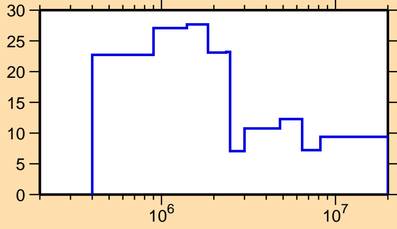
\Delta\sigma/\sigma vs. E for ^{96}\text{Tc}(n,el.)
