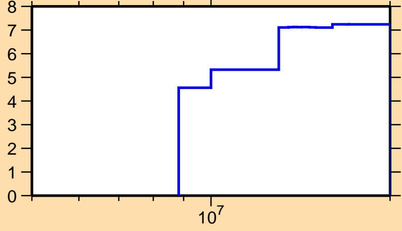
\Delta\sigma/\sigma vs. E for ^{97}\text{Tc}(n,\text{tot.})
