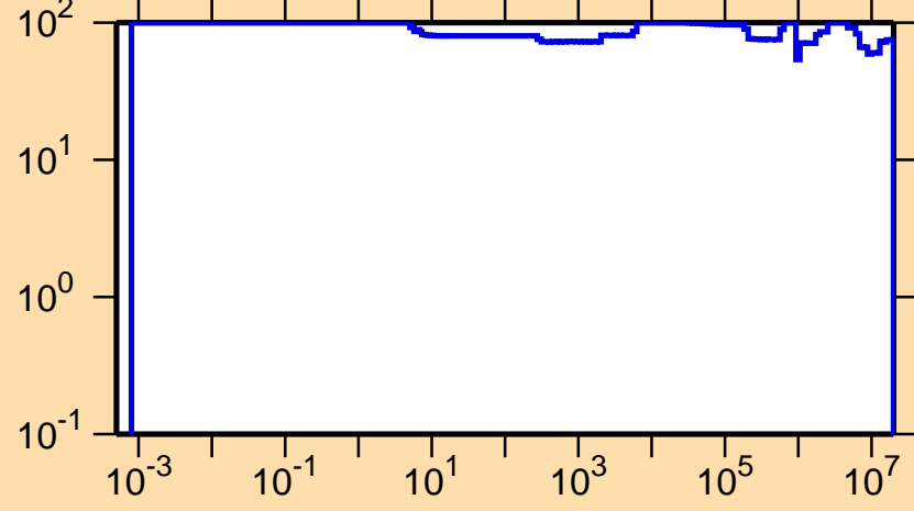
\Delta\sigma/\sigma vs. E for ^{97}\text{Tc}(n,p)
