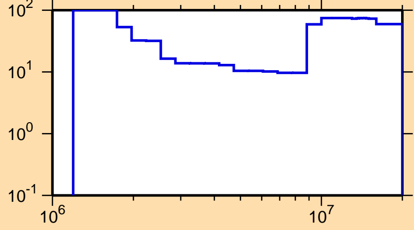
\Delta\sigma/\sigma vs. E for ^{97}\text{Tc}(n,n\text{cont.})
