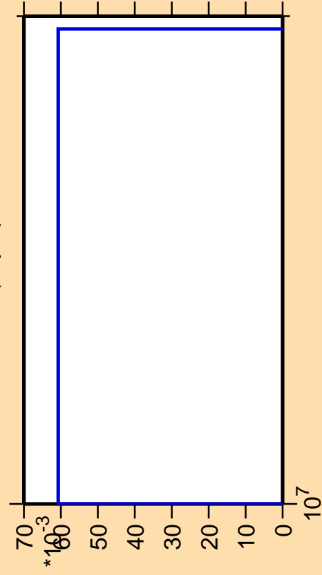
\Delta\sigma/\sigma vs. E for ^{97}\text{Tc}(n,pd)
