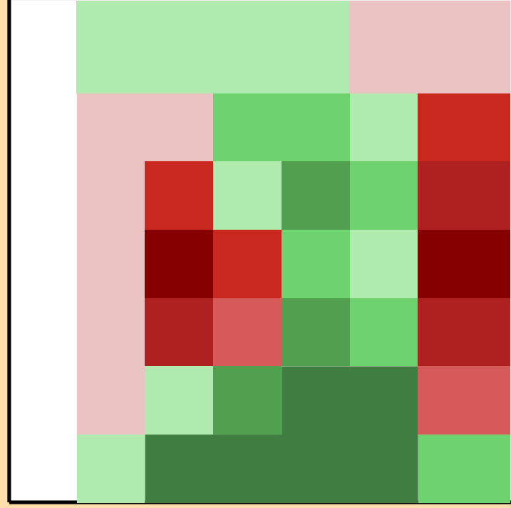
\Delta\sigma/\sigma vs. E for ^{97}\text{Tc}(n,n\text{cont.})
