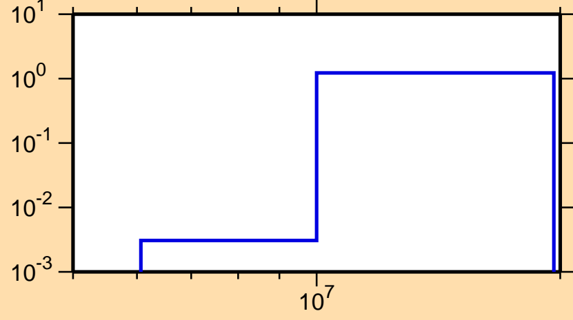
\sigma vs. E for ^{97}\text{Tc}(n,2n)
