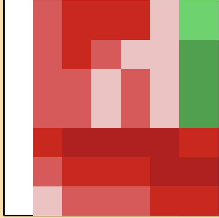
\Delta\sigma/\sigma vs. E for ^{97}\text{Tc}(n,ncont.)
