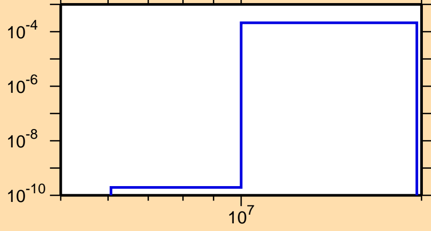
\sigma vs. E for ^{97}\text{Tc}(n,t)
