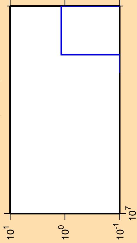
\Delta\sigma/\sigma vs. E for ^{100}\text{Tc}(\text{mt117})
