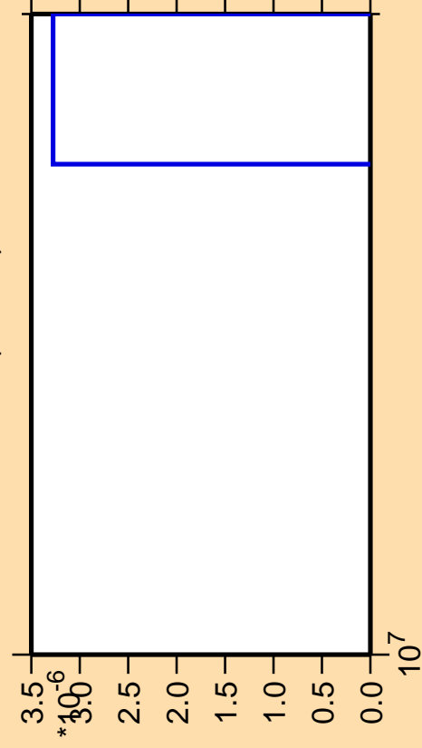
\Delta\sigma/\sigma vs. E for ^{100}\text{Tc} (mt 11)
