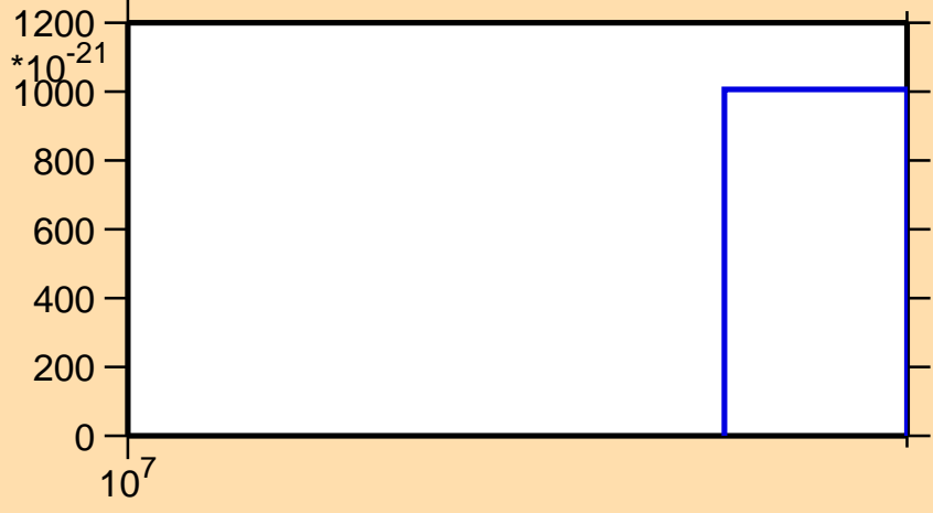
\sigma vs. E for ^{100}\text{Tc} (mt 11)
