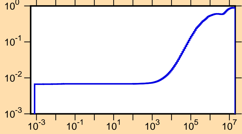
\mu vs. E for ^{101}\text{Tc}(\text{mt251})
