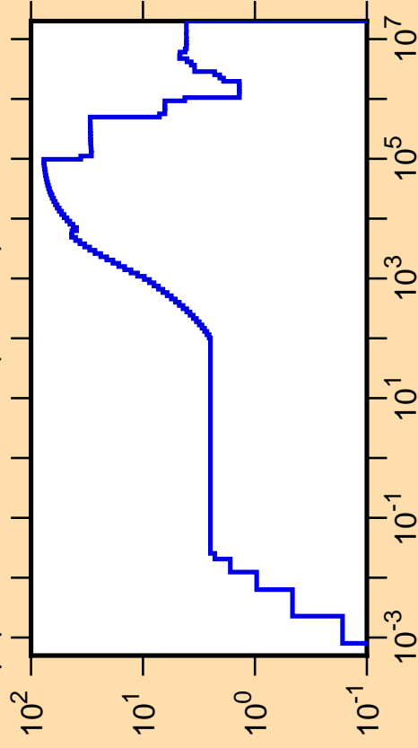
\Delta\mu/\mu vs. E for ^{101}\text{Tc}(\text{mt251})
