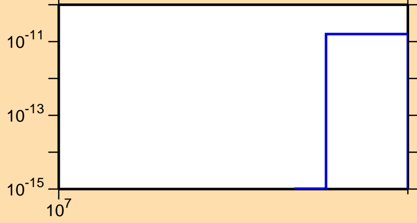
\sigma vs. E for ^{101}\text{Tc}(n,\text{He3})
