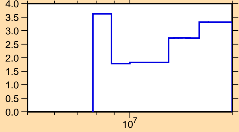
\Delta\sigma/\sigma vs. E for ^{101}\text{Tc}(n,\text{el.})
