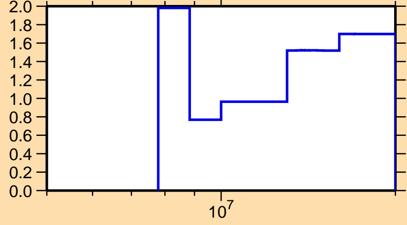
\Delta\sigma/\sigma vs. E for ^{101}\text{Tc}(n,\text{tot.})
