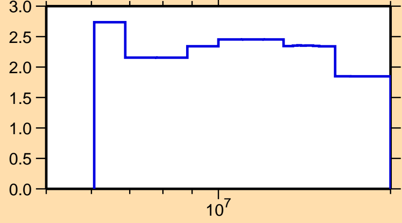
\Delta\sigma/\sigma vs. E for ^{102}\text{Tc}(n,\text{nonel.})
