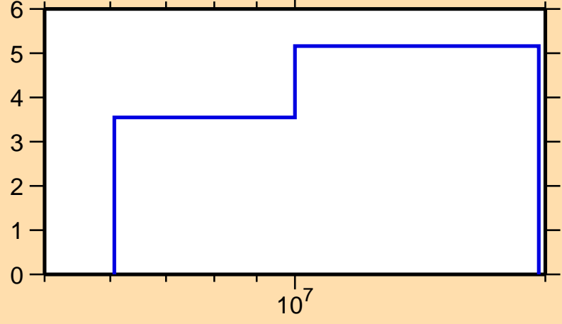
\Delta\sigma/\sigma vs. E for ^{102}\text{Tc}(n,\text{el.})
