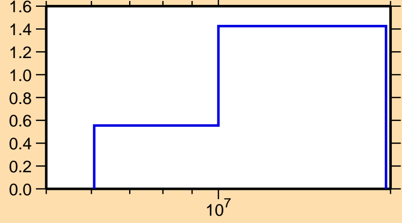
\sigma vs. E for ^{102}\text{Tc}(n,2n)
