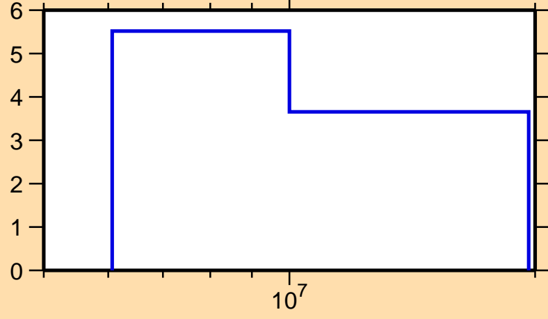
\Delta\sigma/\sigma vs. E for ^{102}\text{Tc}(n,2n)
