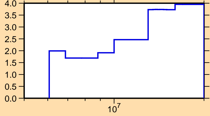
\Delta\sigma/\sigma vs. E for ^{102}\text{Tc}(n,\text{tot.})
