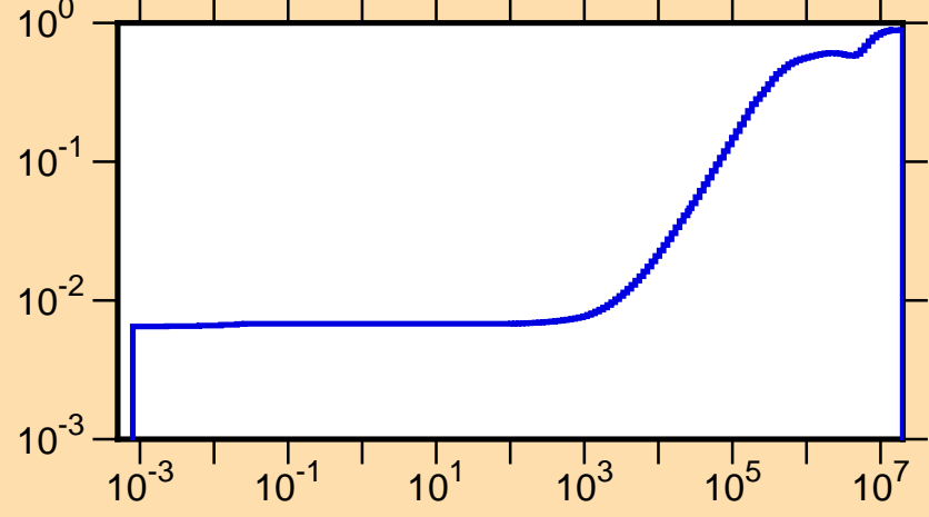
\mu vs. E for ^{104}\text{Tc}(\text{mt251})
