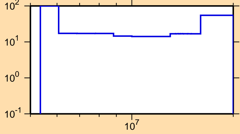
\Delta\sigma/\sigma vs. E for ^{104}\text{Tc}(n,2n)
