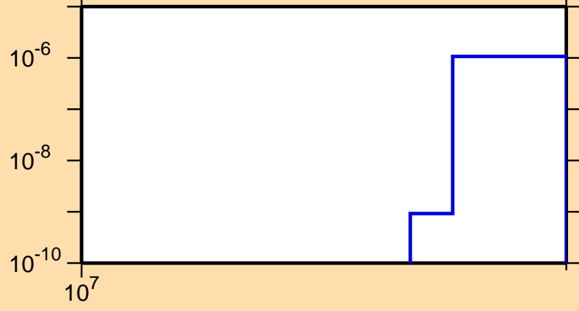
\sigma vs. E for ^{104}\text{Tc}(n,nt)
