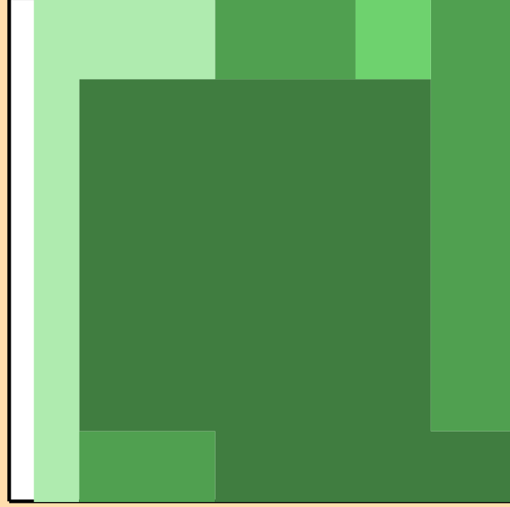
\Delta\sigma/\sigma vs. E for ^{104}\text{Tc}(n,2n)
