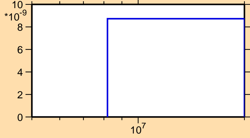
\sigma vs. E for ^{104}\text{Tc}(n,nt)
