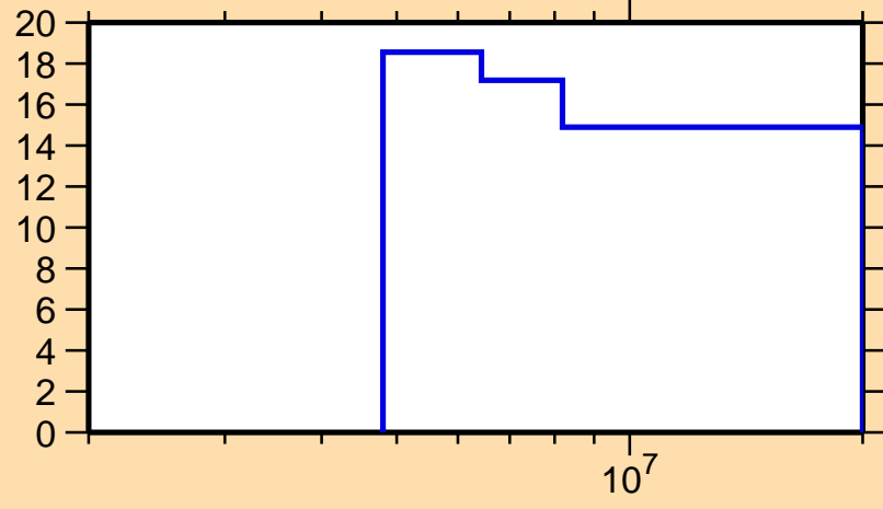
\Delta\sigma/\sigma vs. E for ^{104}\text{Tc}(n,2n)
