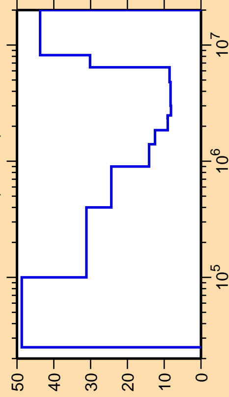
\Delta\sigma/\sigma vs. E for ^{104}\text{Tc}(n,\text{inel.})
