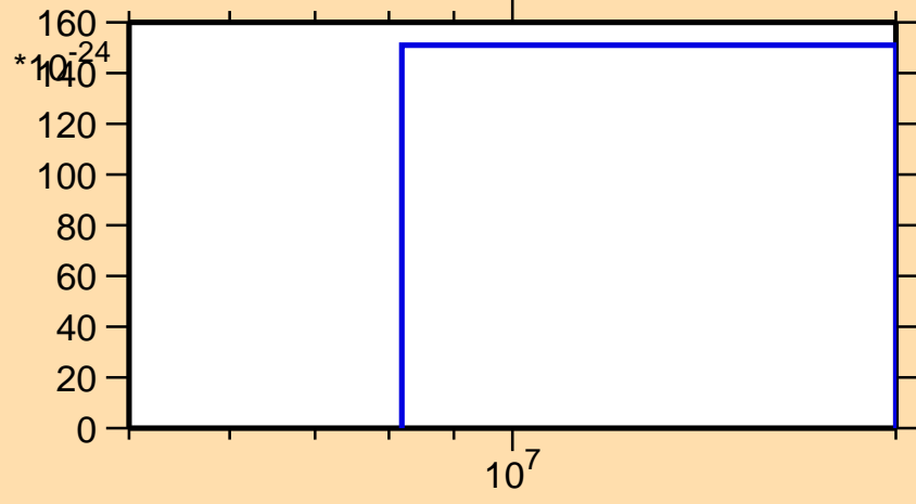
\sigma vs. E for ^{104}\text{Tc}(\text{mt } 34)
