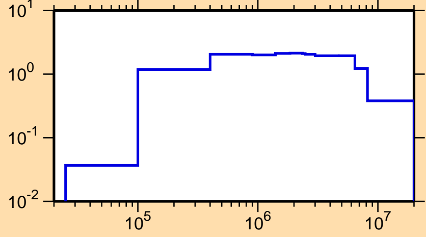
\sigma vs. E for ^{104}\text{Tc}(n,\text{inel.})
