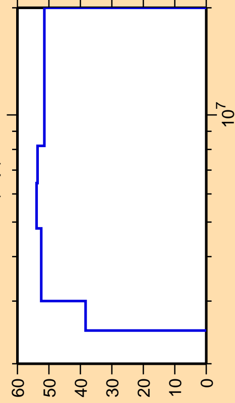
\Delta\sigma/\sigma vs. E for ^{104}\text{Tc}(n,p)
