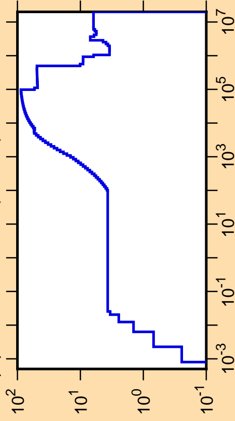
\Delta\mu/\mu vs. E for ^{105}\text{Tc}(\text{mt251})
