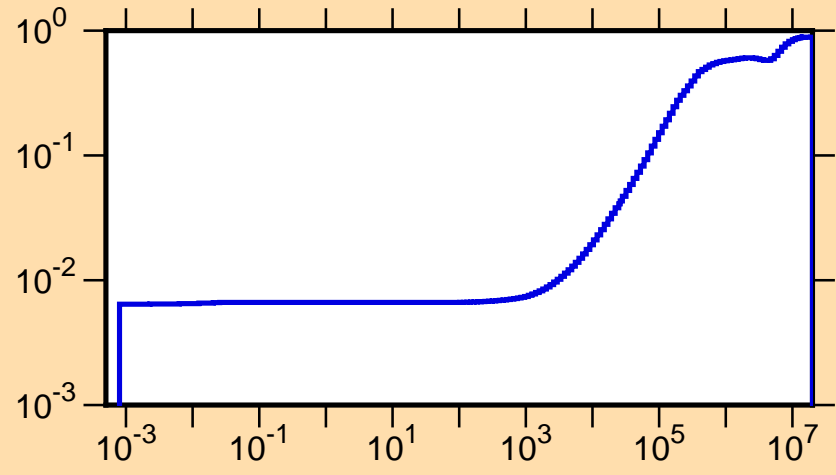
\mu vs. E for ^{105}\text{Tc}(\text{mt251})
