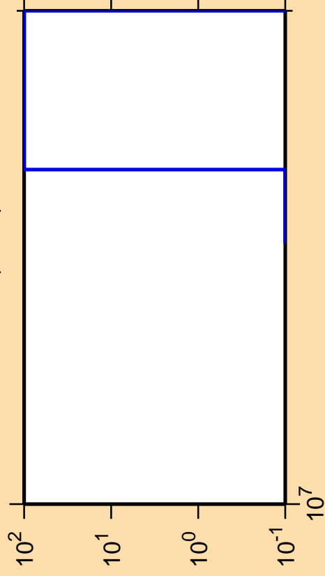
\Delta\sigma/\sigma vs. E for ^{105}\text{Tc}(n,nd)
