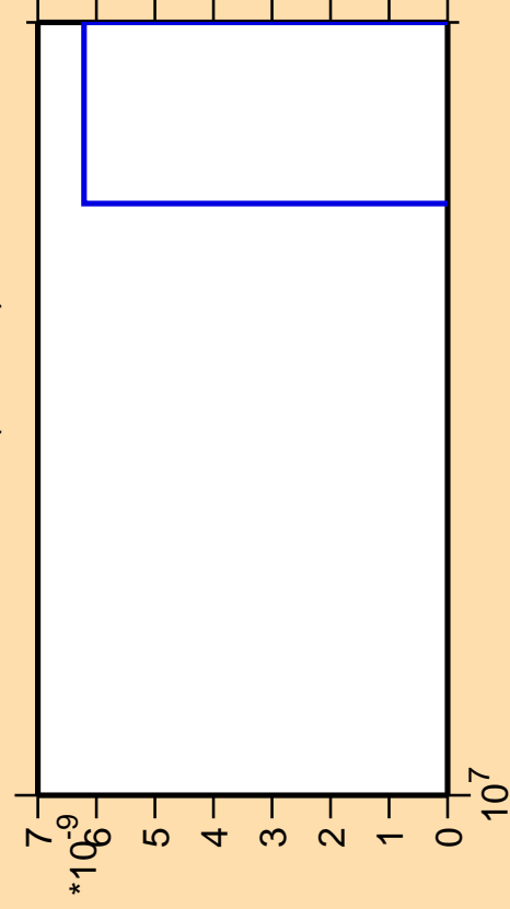
\Delta\sigma/\sigma vs. E for ^{105}\text{Tc}(n,3n\alpha)
