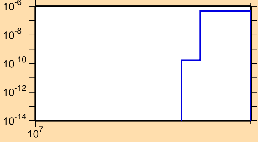
\sigma vs. E for ^{105}\text{Tc}(n,nd)
