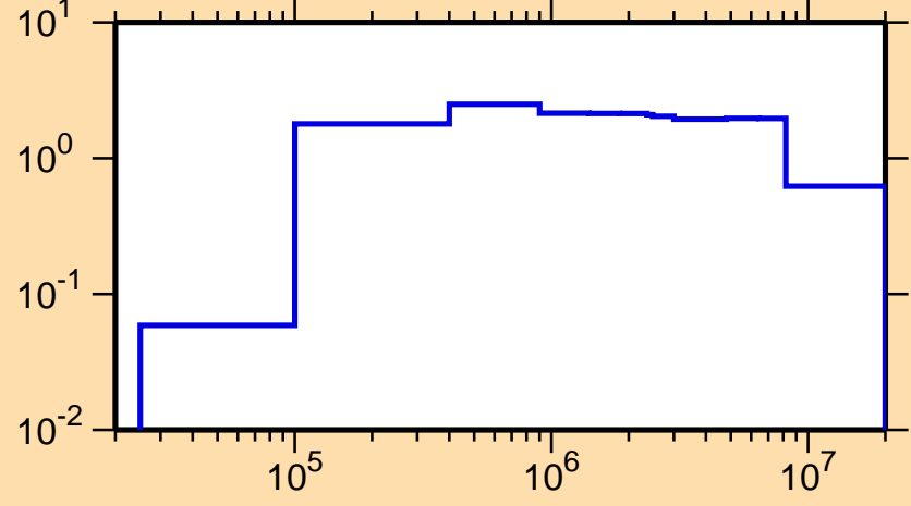
\sigma vs. E for ^{105}\text{Tc}(n,\text{inel.})
