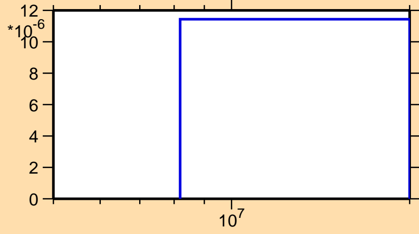
\sigma vs. E for ^{105}\text{Tc}(n,t)
