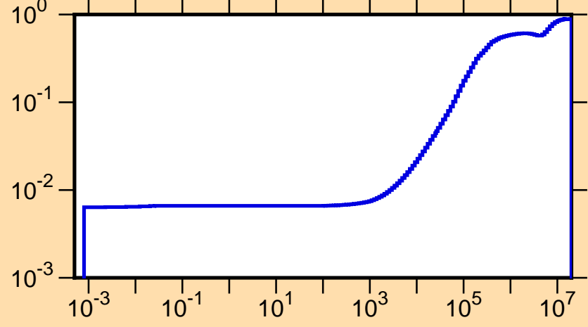
\mu vs. E for ^{106}\text{Tc}(\text{mt251})
