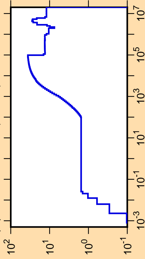
\Delta\mu/\mu vs. E for ^{106}\text{Tc}(\text{mt251})
