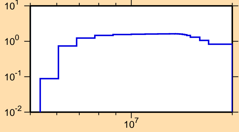
\sigma vs. E for ^{106}\text{Tc}(n,2n)
