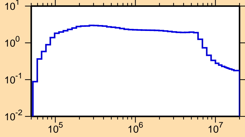
\sigma vs. E for ^{106}\text{Tc}(n,\text{inel.})
