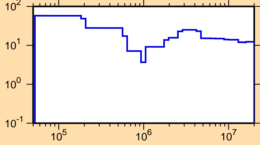
\Delta\sigma/\sigma vs. E for ^{106}\text{Tc}(n,\text{nonel.})
