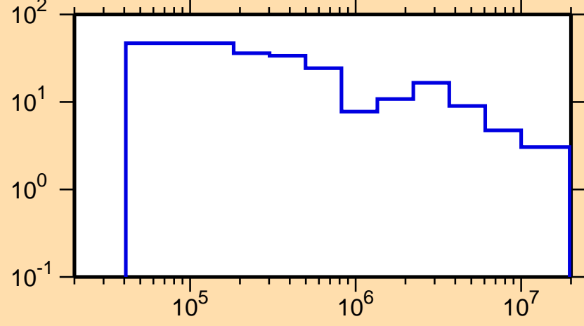
\Delta\sigma/\sigma vs. E for ^{106}\text{Tc}(n,\text{tot.})
