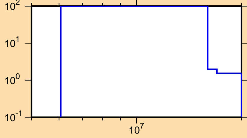
\Delta\sigma/\sigma vs. E for ^{108}\text{Tc}(n,n_1)
