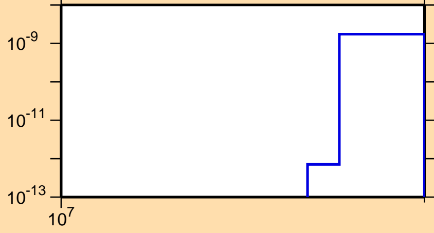
\sigma vs. E for ^{108}\text{Tc}(n,2n\alpha)
