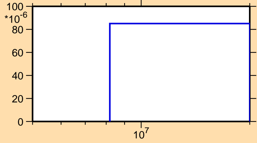
\sigma vs. E for ^{108}\text{Tc}(n,d)
