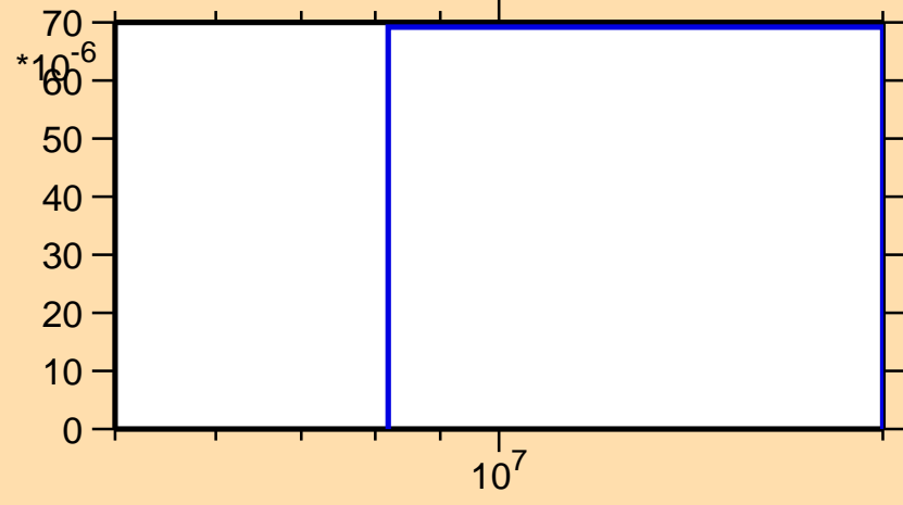
\sigma vs. E for ^{109}\text{Tc}(n,d)
