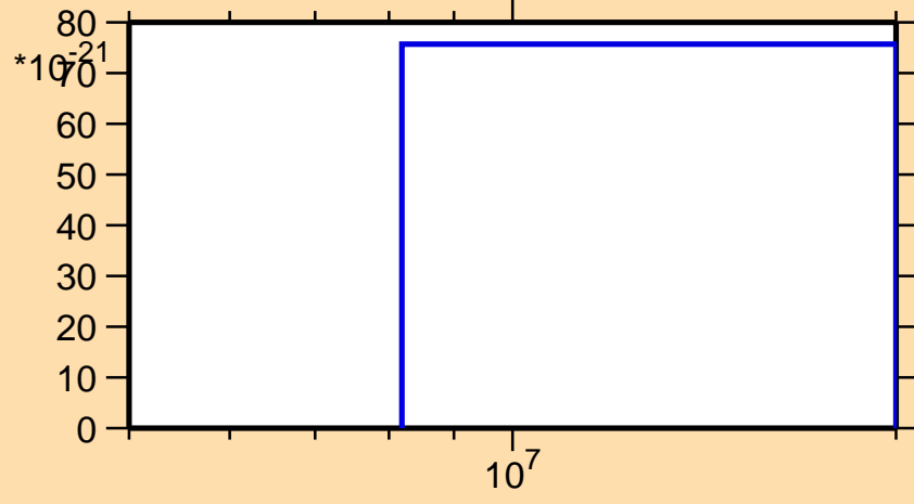
\sigma vs. E for ^{109}\text{Tc}(\text{mt } 11)
