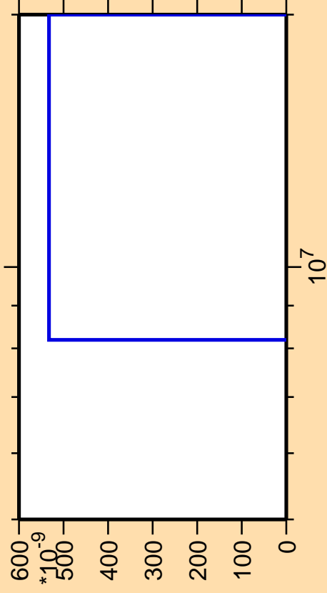
\Delta\sigma/\sigma vs. E for ^{109}\text{Tc}(\text{mt } 11)
