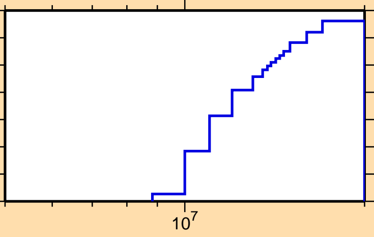
\sigma vs. E for ^{110}\text{Te}(\text{mt117})
