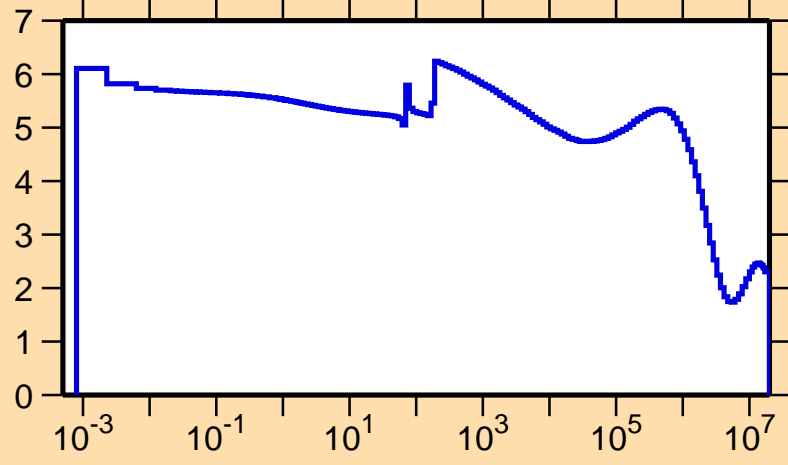
\sigma vs. E for ^{110}\text{Te}(n,\text{el.})
