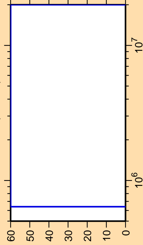
\Delta\sigma/\sigma vs. E for ^{110}\text{Te}(n,\text{inel.})
