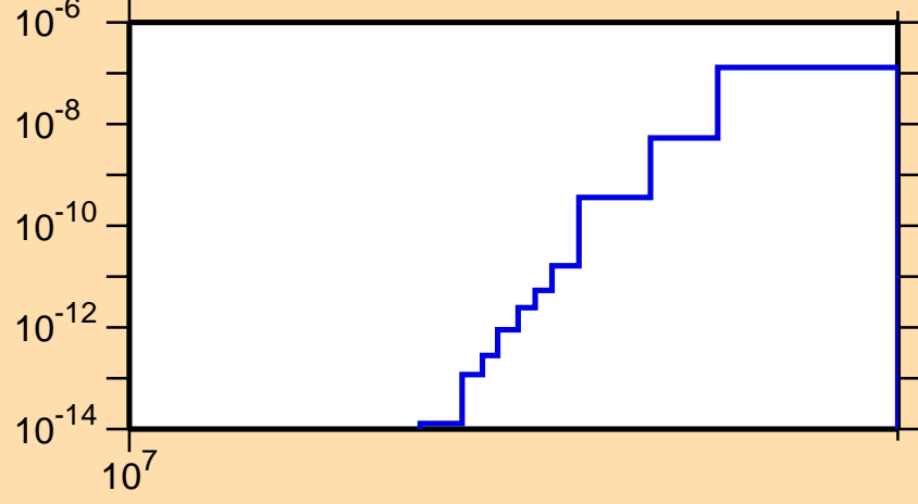
\sigma vs. E for ^{110}\text{Te} (mt 34)
