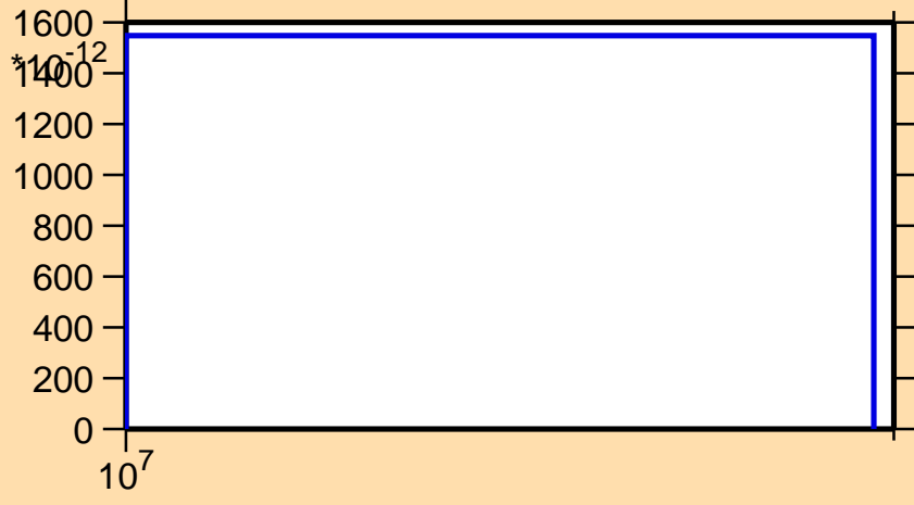
\sigma vs. E for ^{110}\text{Te}(n,nd)
