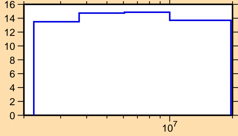
\Delta\sigma/\sigma vs. E for ^{110}\text{Te}(n,n\text{nonel.})
