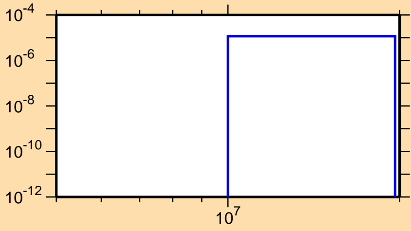
\sigma vs. E for ^{110}\text{Te}(\text{mt } 45)
