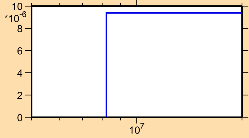
\sigma vs. E for ^{110}\text{Te}(\text{mt } 45)
