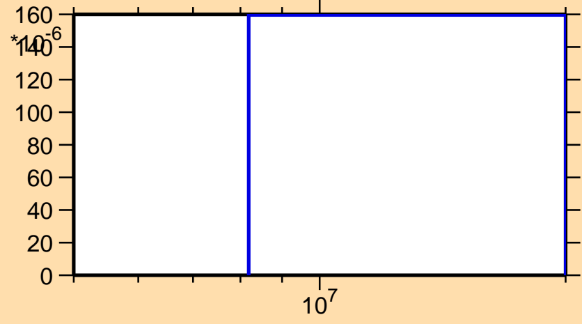
\sigma vs. E for ^{110}\text{Te}(n,t)
