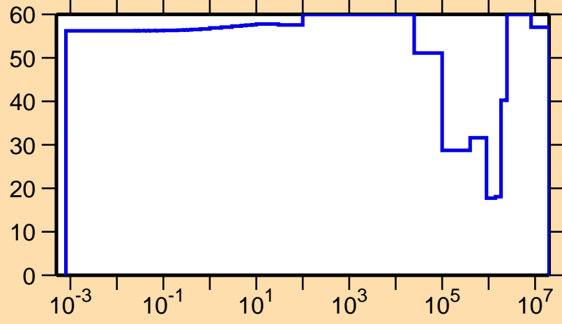
\Delta\sigma/\sigma vs. E for ^{110}\text{Te}(n,\text{el.})
