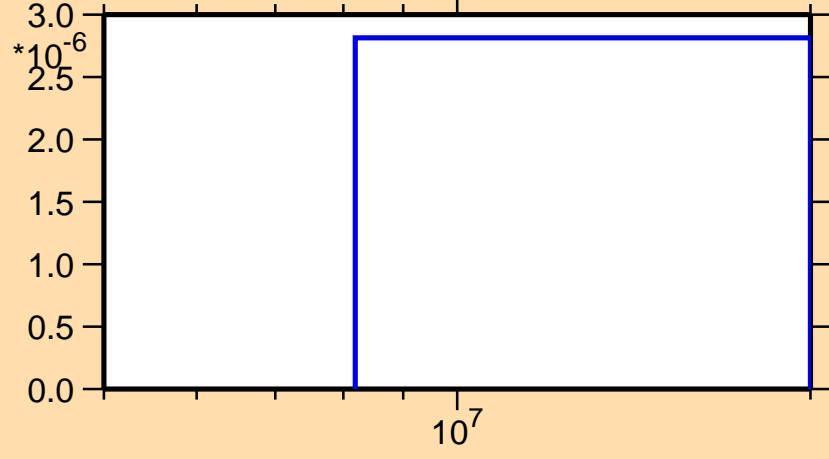
\sigma vs. E for ^{110}\text{Te}(n,\text{pt})
