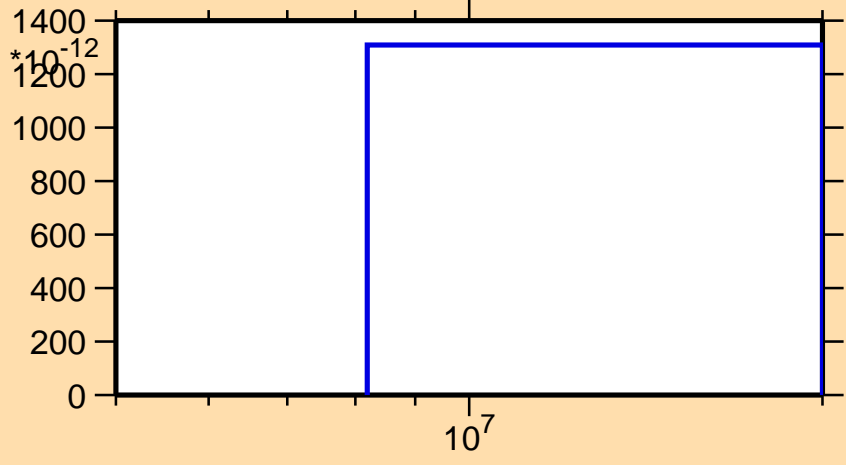
\sigma vs. E for ^{110}\text{Te}(\text{mt } 34)
