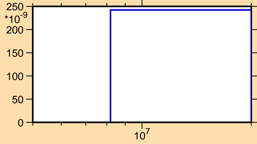
\sigma vs. E for ^{110}\text{Te}(\text{mt117})
