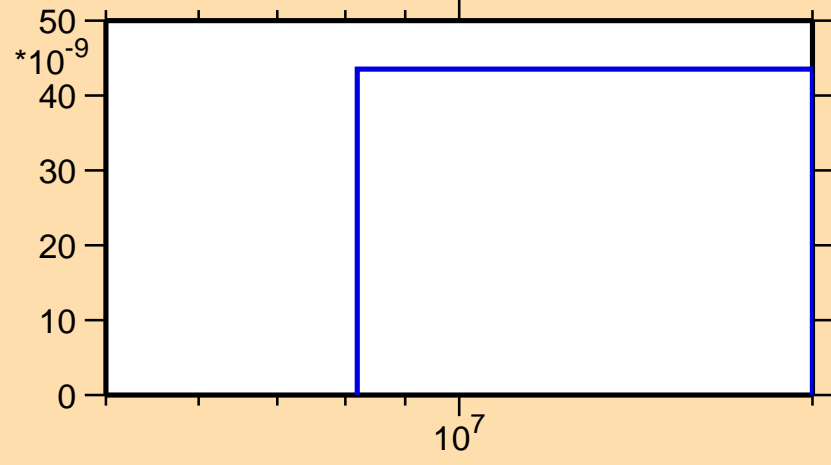
\sigma vs. E for ^{110}\text{Te}(n,2n\alpha)
