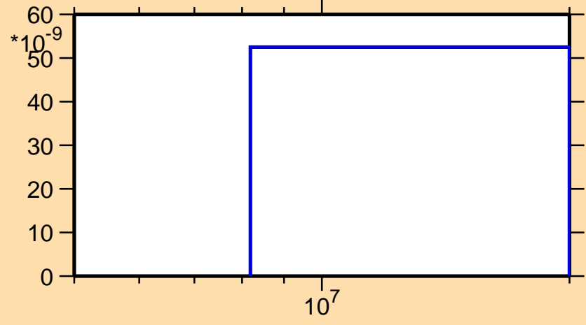
\sigma vs. E for ^{110}\text{Te}(n,2np)
