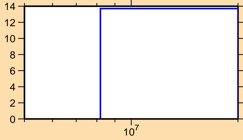
\Delta\sigma/\sigma vs. E for ^{110}\text{Te}(n,\text{nonel.})
