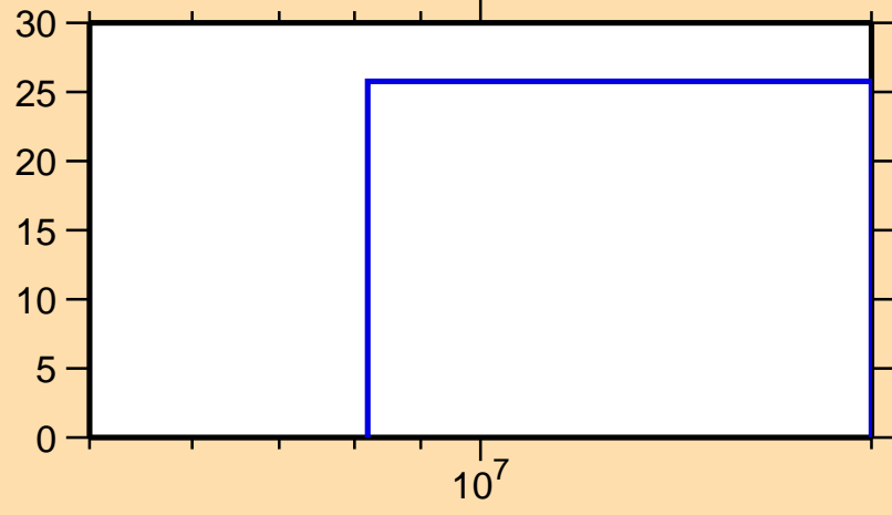
\Delta\sigma/\sigma vs. E for ^{110}\text{Te}(n,\text{tot.})
