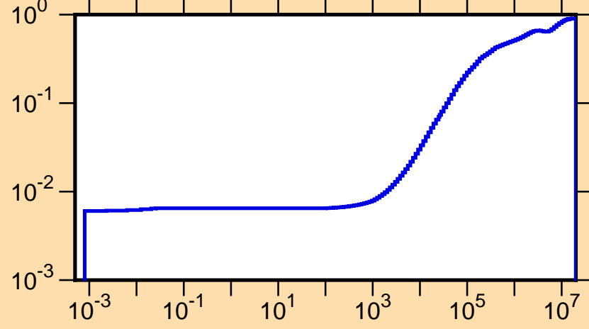
\mu vs. E for ^{112}\text{Te}(\text{mt251})
