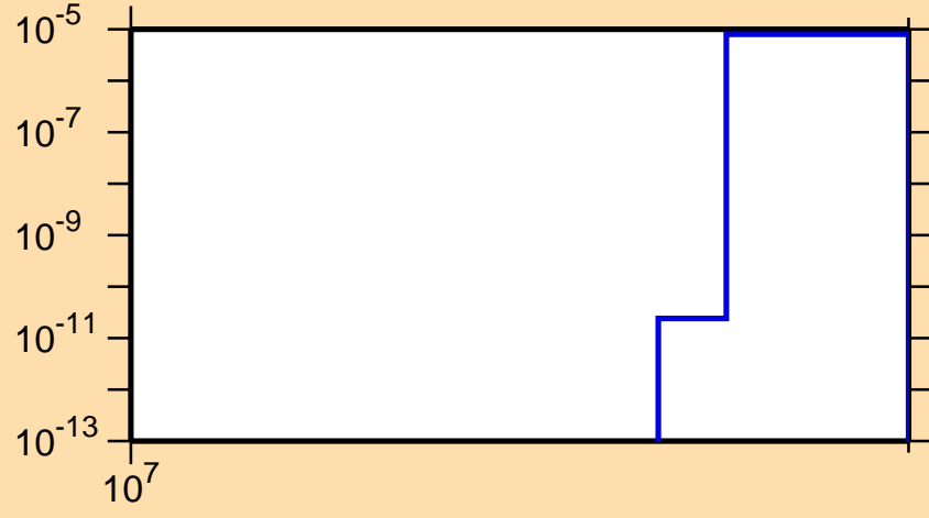
\sigma vs. E for ^{112}\text{Te}(n,2np)
