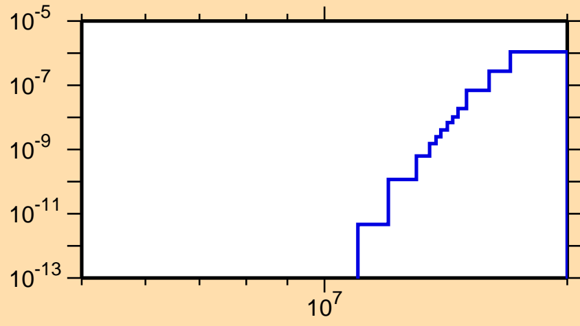
\sigma vs. E for ^{112}\text{Te}(\text{mt117})
