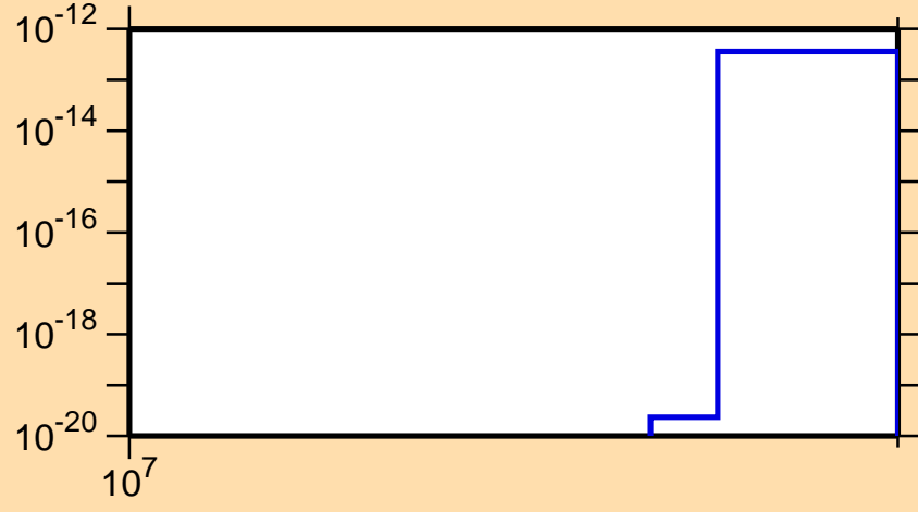
\sigma vs. E for ^{112}\text{Te}(n,nt)
