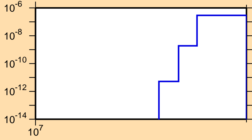
\sigma vs. E for ^{112}\text{Te}(n,\text{nd})
