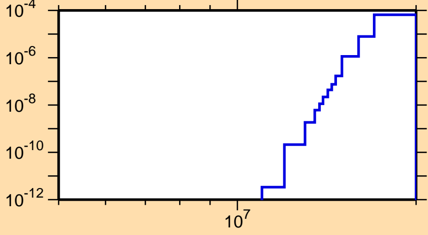
\sigma vs. E for ^{112}\text{Te}(\text{mt } 45)
