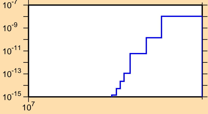
\sigma vs. E for ^{112}\text{Te} (mt 34)
