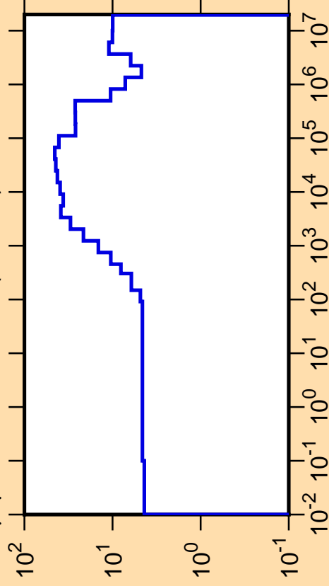
\Delta\mu/\mu vs. E for ^{112}\text{Te}(\text{mt251})
