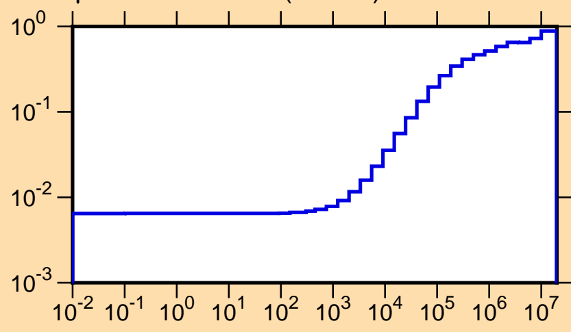
\mu vs. E for ^{112}\text{Te}(\text{mt251})
