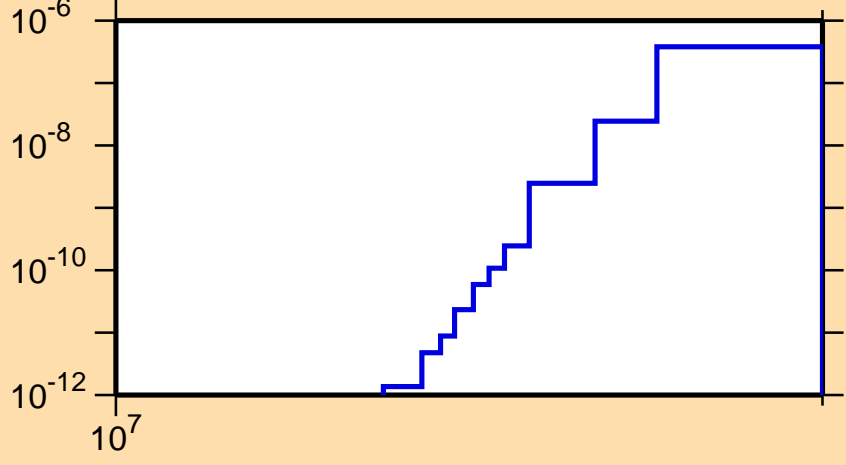
\sigma vs. E for ^{113}\text{Te} (mt 34)
