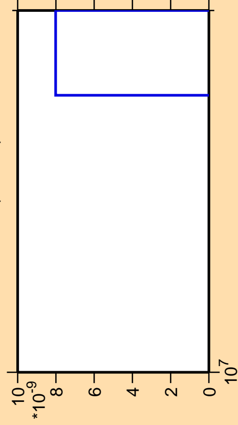
\Delta\sigma/\sigma vs. E for ^{113}\text{Te}(n,3n\alpha)
