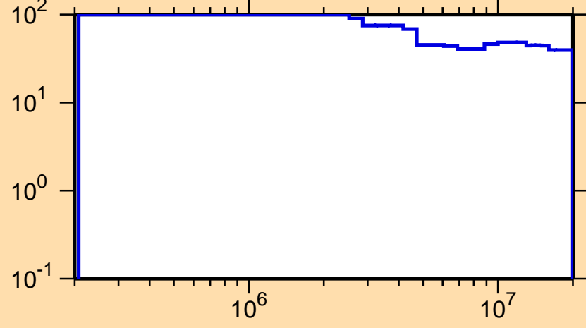
\Delta\sigma/\sigma vs. E for ^{113}\text{Te}(n,n_1)
