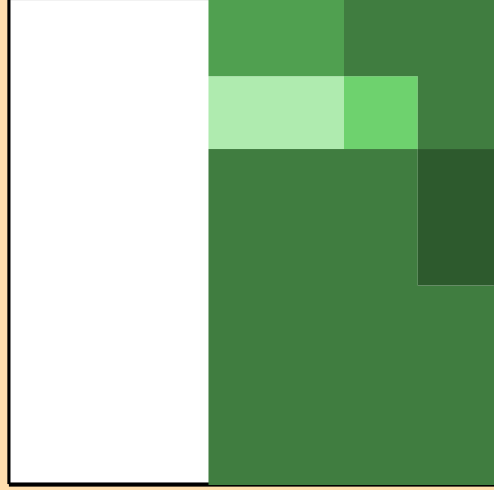
\Delta\sigma/\sigma vs. E for ^{113}\text{Te}(n,2n)
