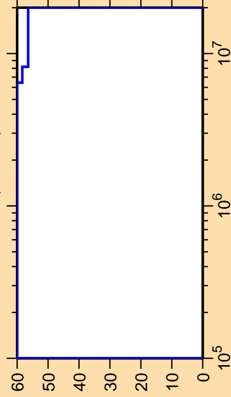
\Delta\sigma/\sigma vs. E for ^{113}\text{Te}(n,\text{inel.})
