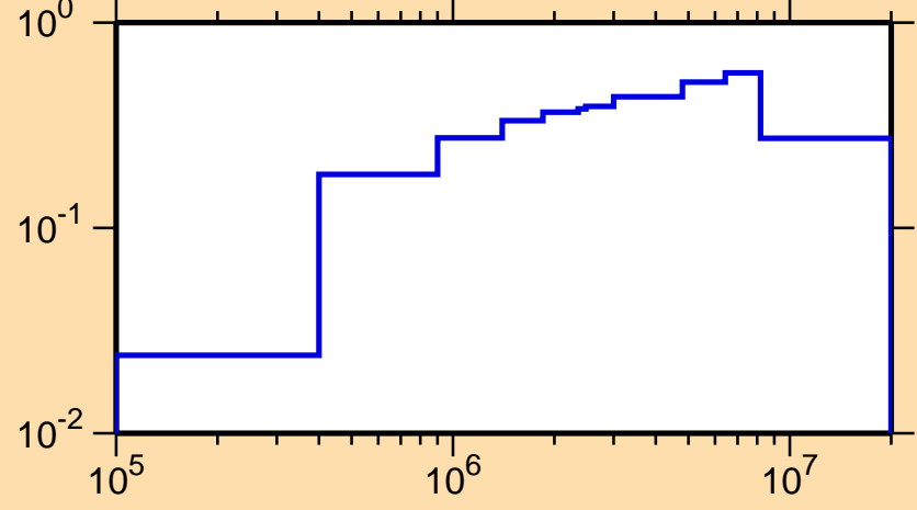
\sigma vs. E for ^{113}\text{Te}(n,\text{inel.})
