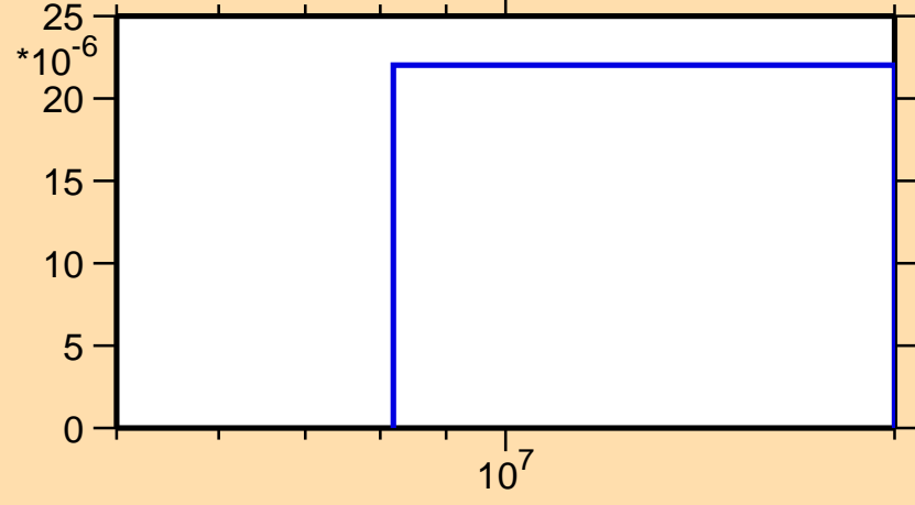
\sigma vs. E for ^{113}\text{Te}(n,2n\alpha)
