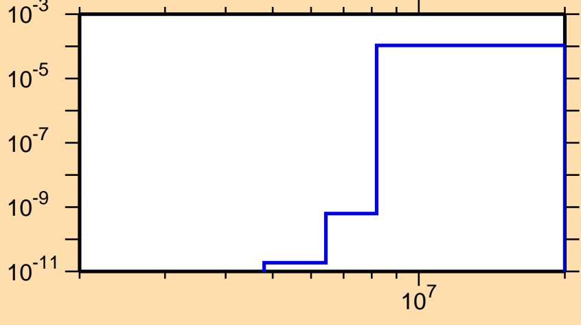
\sigma vs. E for ^{113}\text{Te}(n,\text{He3})
