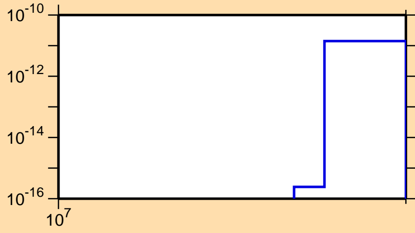
\sigma vs. E for ^{114}\text{Te}(n,nt)
