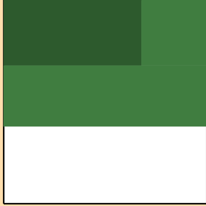
\Delta\sigma/\sigma vs. E for ^{114}\text{Te}(n,\text{nonel.})
