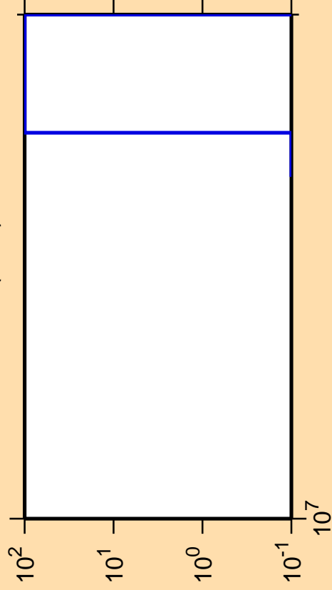
\Delta\sigma/\sigma vs. E for ^{114}\text{Te}(n,nt)
