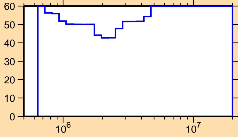
\Delta\sigma/\sigma vs. E for ^{114}\text{Te}(n,n_1)
