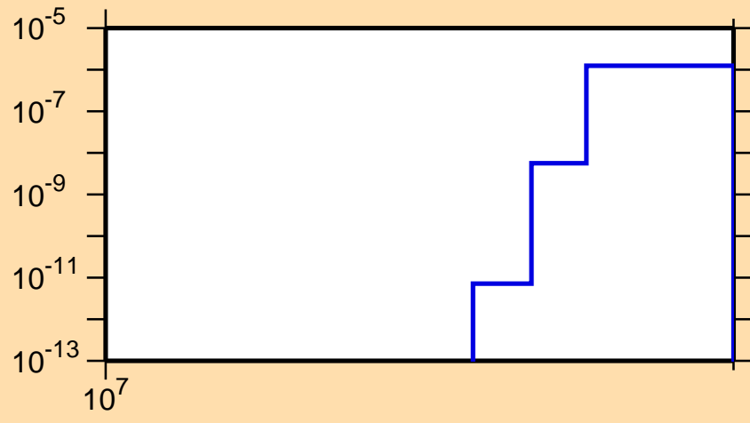
\sigma vs. E for ^{114}\text{Te}(n,\text{nd})
