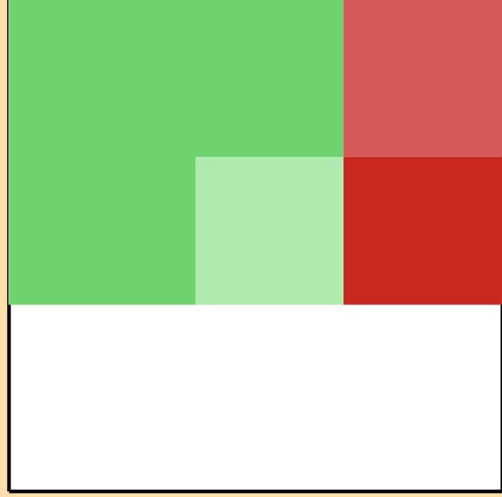
\Delta\sigma/\sigma vs. E for ^{114}\text{Te}(n,\text{el.})
