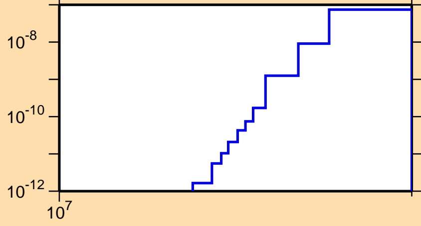
\sigma vs. E for ^{114}\text{Te}(\text{mt117})
