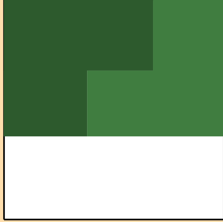
\Delta\sigma/\sigma vs. E for ^{114}\text{Te}(n,\text{inel.})
