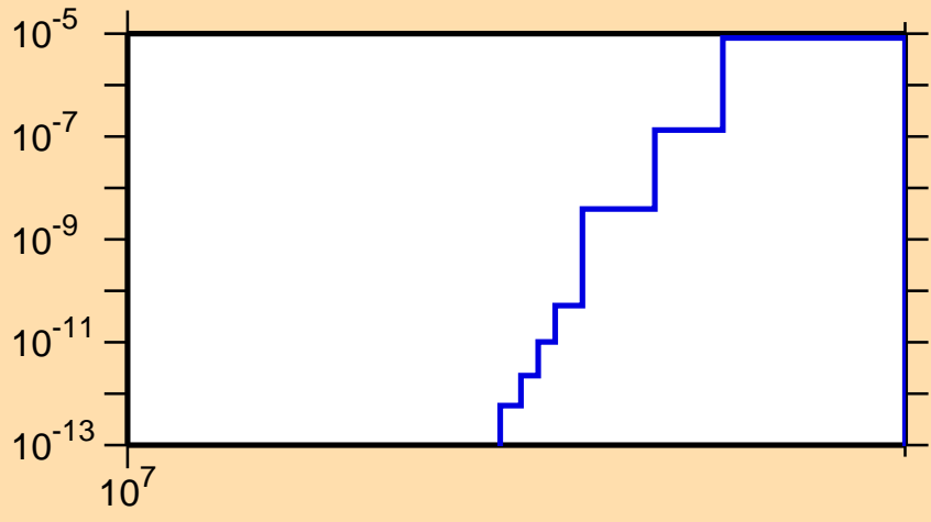
\sigma vs. E for ^{114}\text{Te}(n,2n\alpha)
