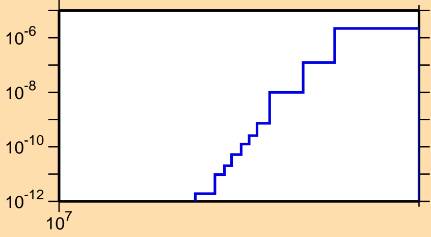
\sigma vs. E for ^{114}\text{Te} (mt 45)
