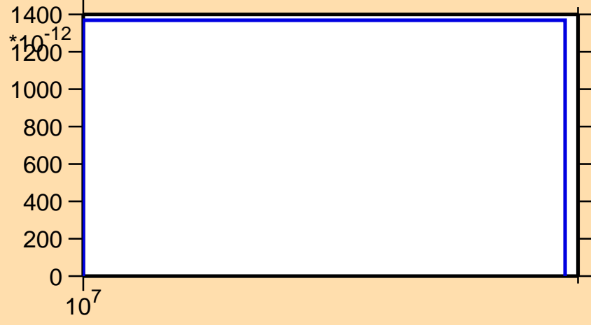
\sigma vs. E for ^{114}\text{Te}(\text{mt117})
