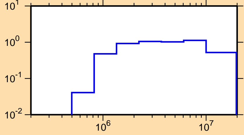
\sigma vs. E for ^{114}\text{Te}(n,\text{inel.})
