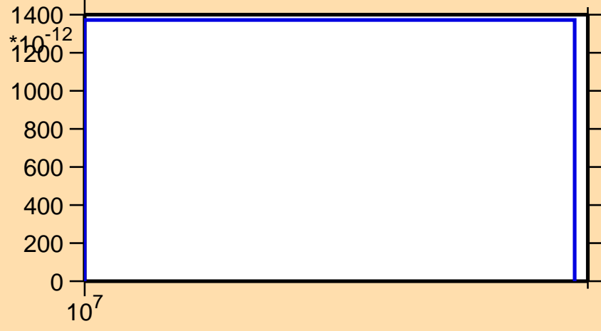
\sigma vs. E for ^{114}\text{Te}(n,\text{pt})
