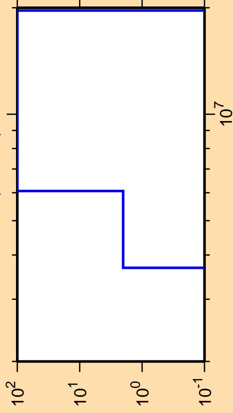
\Delta\sigma/\sigma vs. E for ^{114}\text{Te}(n,\text{He3})
