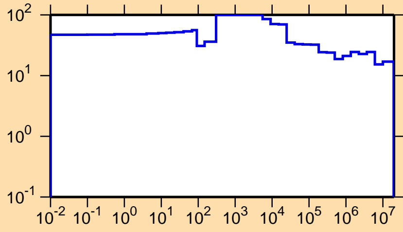
\Delta\sigma/\sigma vs. E for ^{114}\text{Te}(n,\text{el.})
