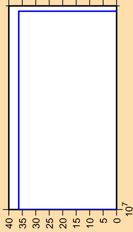
\Delta\sigma/\sigma vs. E for ^{114}\text{Te} (mt 34)
