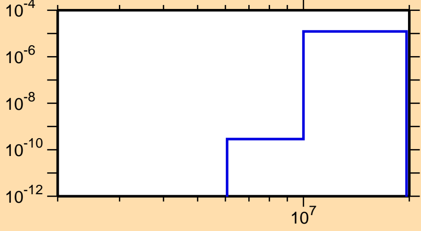
\sigma vs. E for ^{114}\text{Te}(n,\text{He3})
