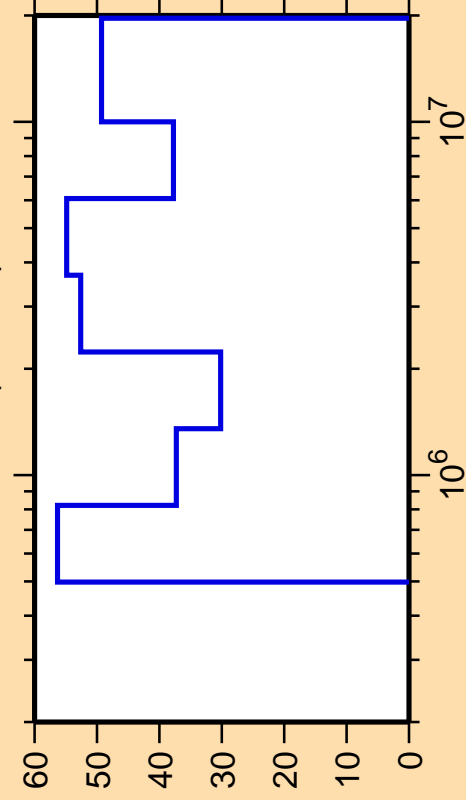
\Delta\sigma/\sigma vs. E for ^{114}\text{Te}(n,\text{inel.})
