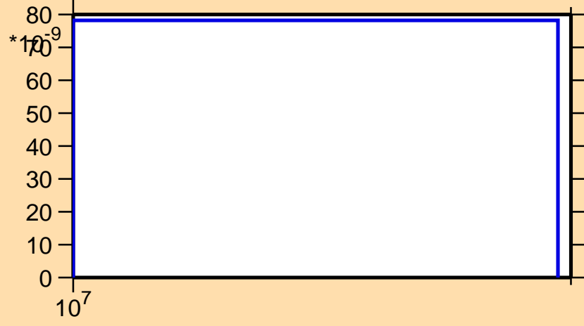
\sigma vs. E for ^{114}\text{Te}(n,2n\alpha)
