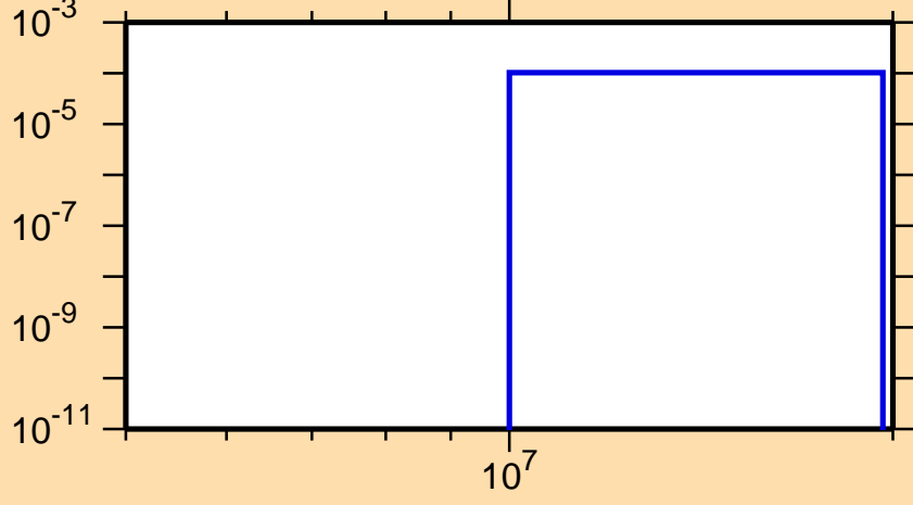
\sigma vs. E for ^{114}\text{Te}(n,t)
