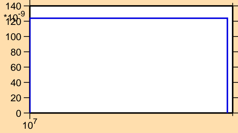
\sigma vs. E for ^{114}\text{Te}(n,2np)
