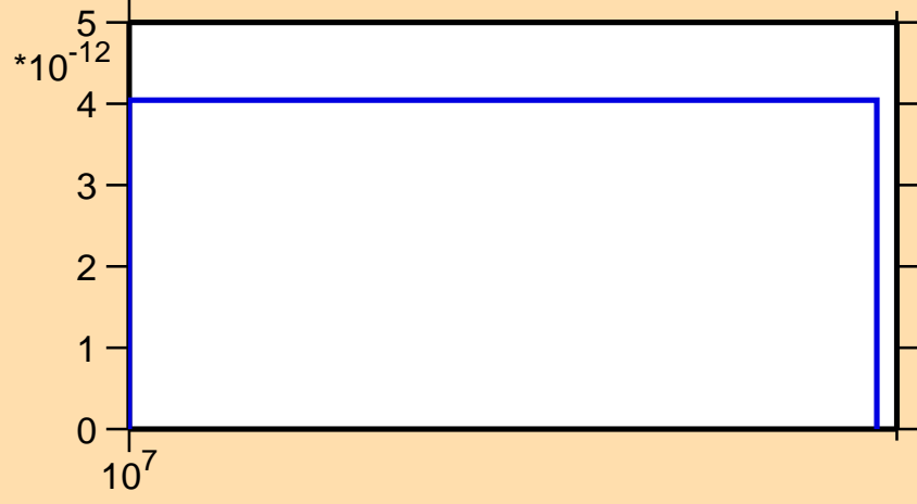
\sigma vs. E for ^{114}\text{Te} (mt 34)
