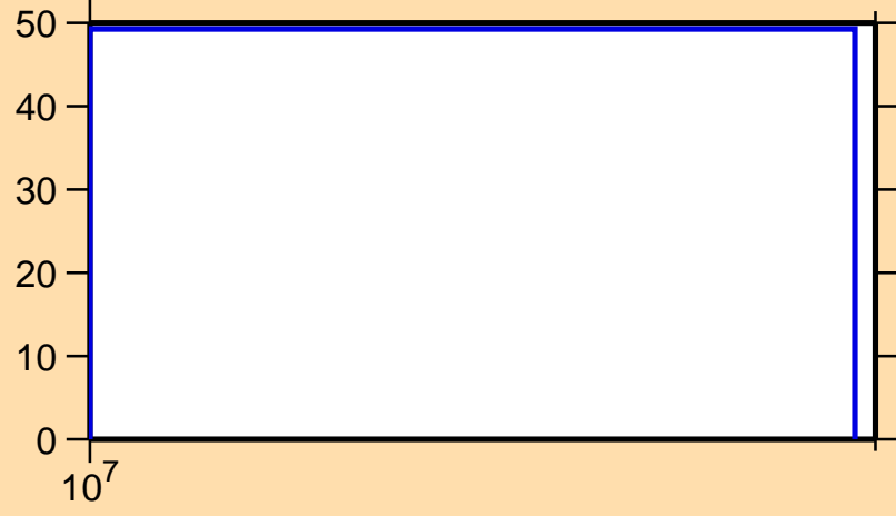
\Delta\sigma/\sigma vs. E for ^{114}\text{Te}(n,\text{inel.})
