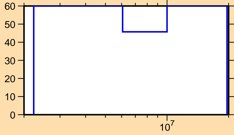
\Delta\sigma/\sigma vs. E for ^{114}\text{Te}(n,n\text{cont.})
