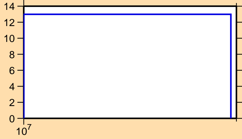
\Delta\sigma/\sigma vs. E for ^{114}\text{Te}(n,\text{nonel.})
