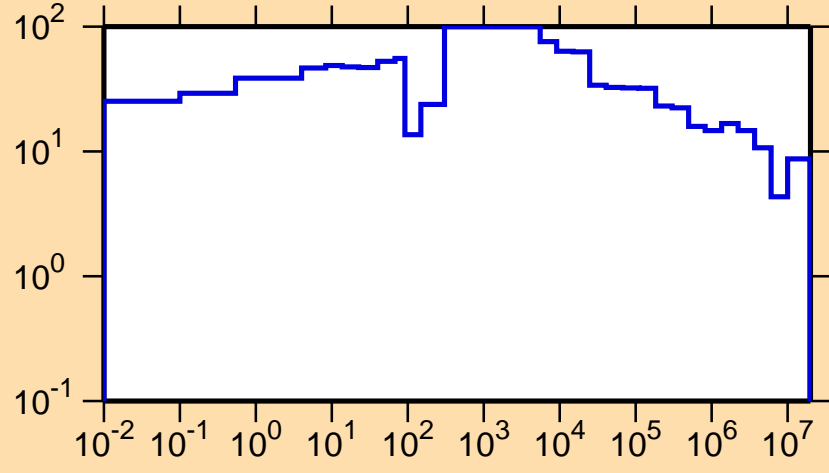
\Delta\sigma/\sigma vs. E for ^{114}\text{Te}(n,\text{tot.})
